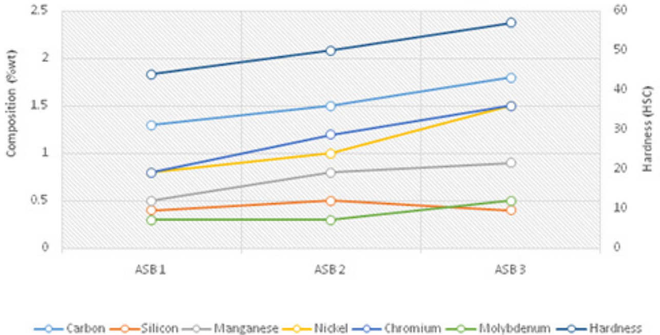
Graph 1: Hardness Vs Chemical composition of Adamite Rolls, ASB: Alloy Steel Base
